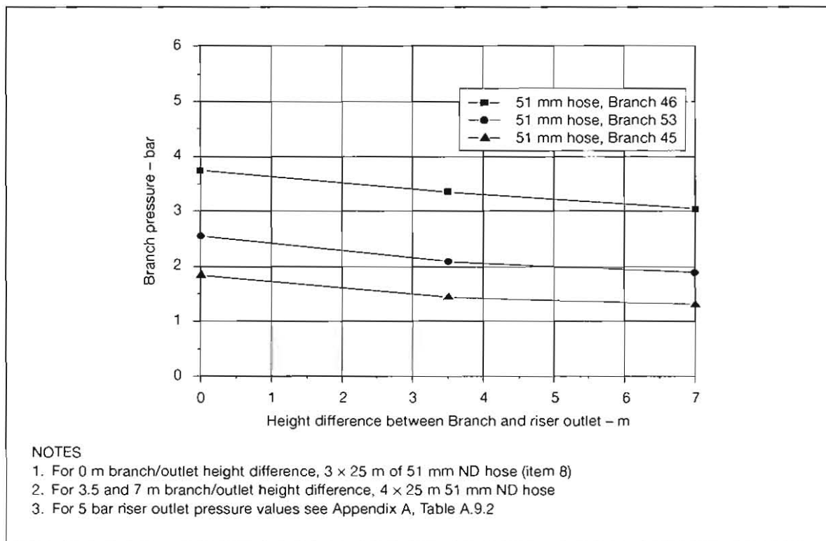
Figure 14. Maximum branch pressures vs. height difference between branch and riser outlet, 4 bar riser outlet pressure, 51 mm hose
