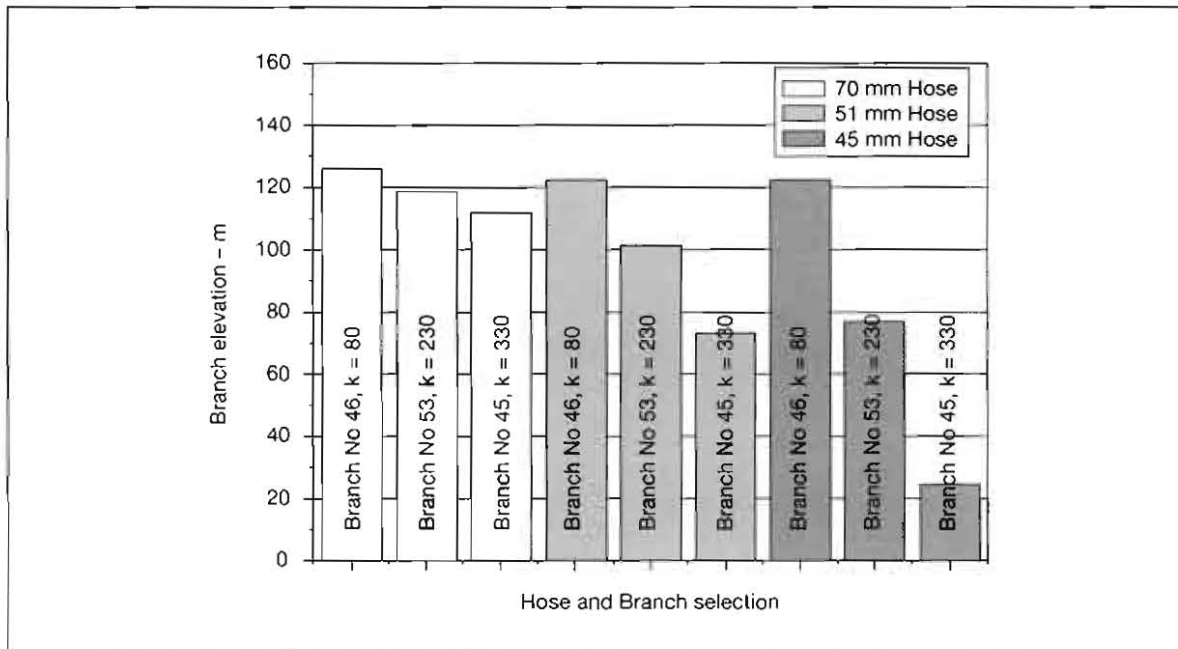
Figure 8. Maximum branch elevation for a branch pressure of 4 bar 3 × 25 m hose lengths
