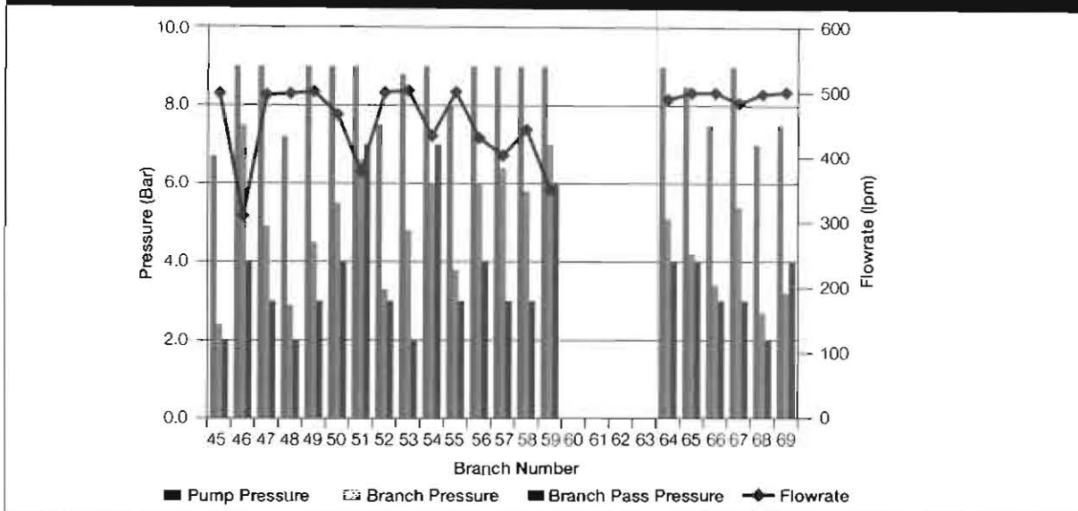
Figure 11: Pressure required to generate a flow of 500 litres/min through 69m of 45mm hose with branches under assessment
