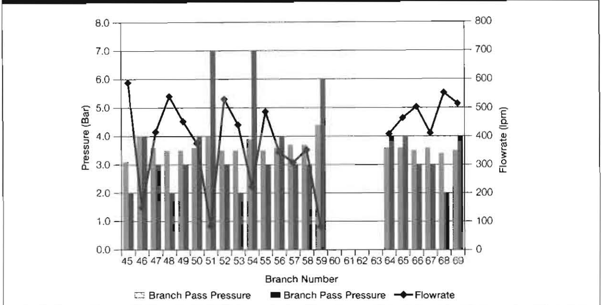
Figure 9: Recorded branch pressure, corresponding branch pass pressure and flowrate when supplied through 69m of 70mm hose at 4 bars pump pressure.
