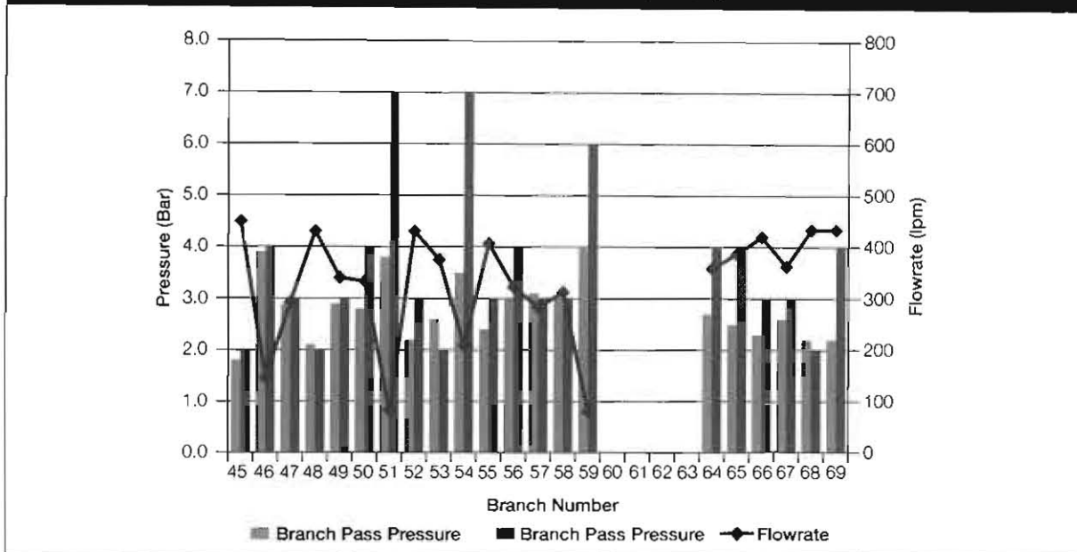
Figure 7: Recorded branch pressure, corresponding branch pass pressure and flowrate when supplied through 69m of 51mm hose at 4 bars pump pressure
