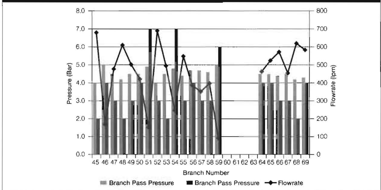
Figure 10: Recorded branch pressure, corresponding branch pass pressure and flowrate when supplied through 69m of 70mm hose at 5 bars pump pressure.
