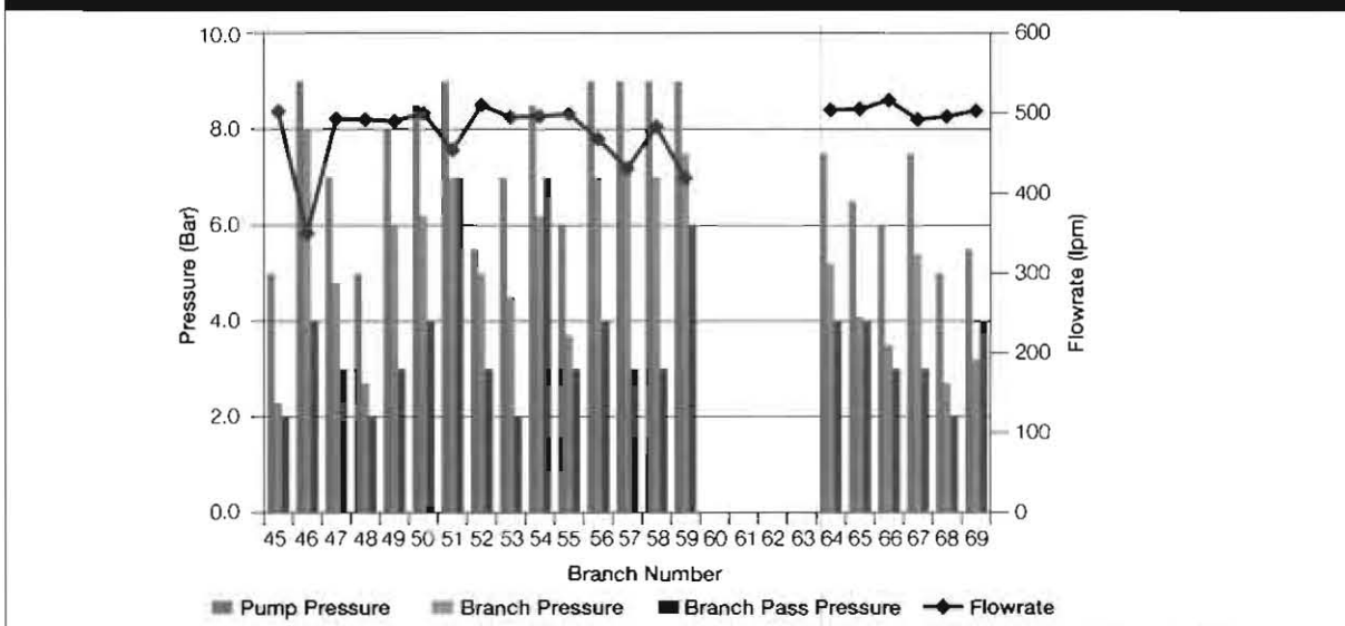
Figure 12: Pressure required to generate a flow of 500 litres/min through 69m of 51 mm hose with branches under assessment
