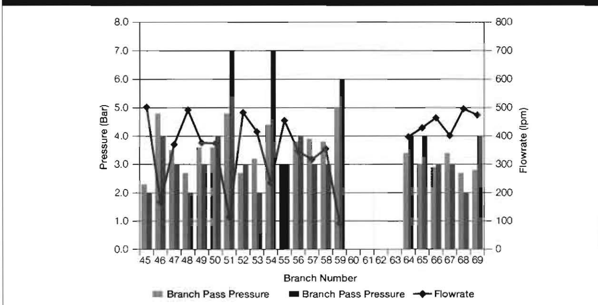
Figure 8: Recorded branch pressure, corresponding branch pass pressure and flowrate when supplied through 69m of 51mm hose at 5 bars pump pressure
